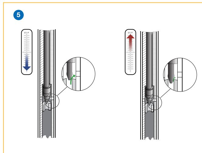
FIGURE 5: Thermal Expansion
